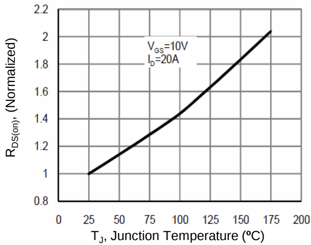
Figure 7. Drain-Source On-Resistance
